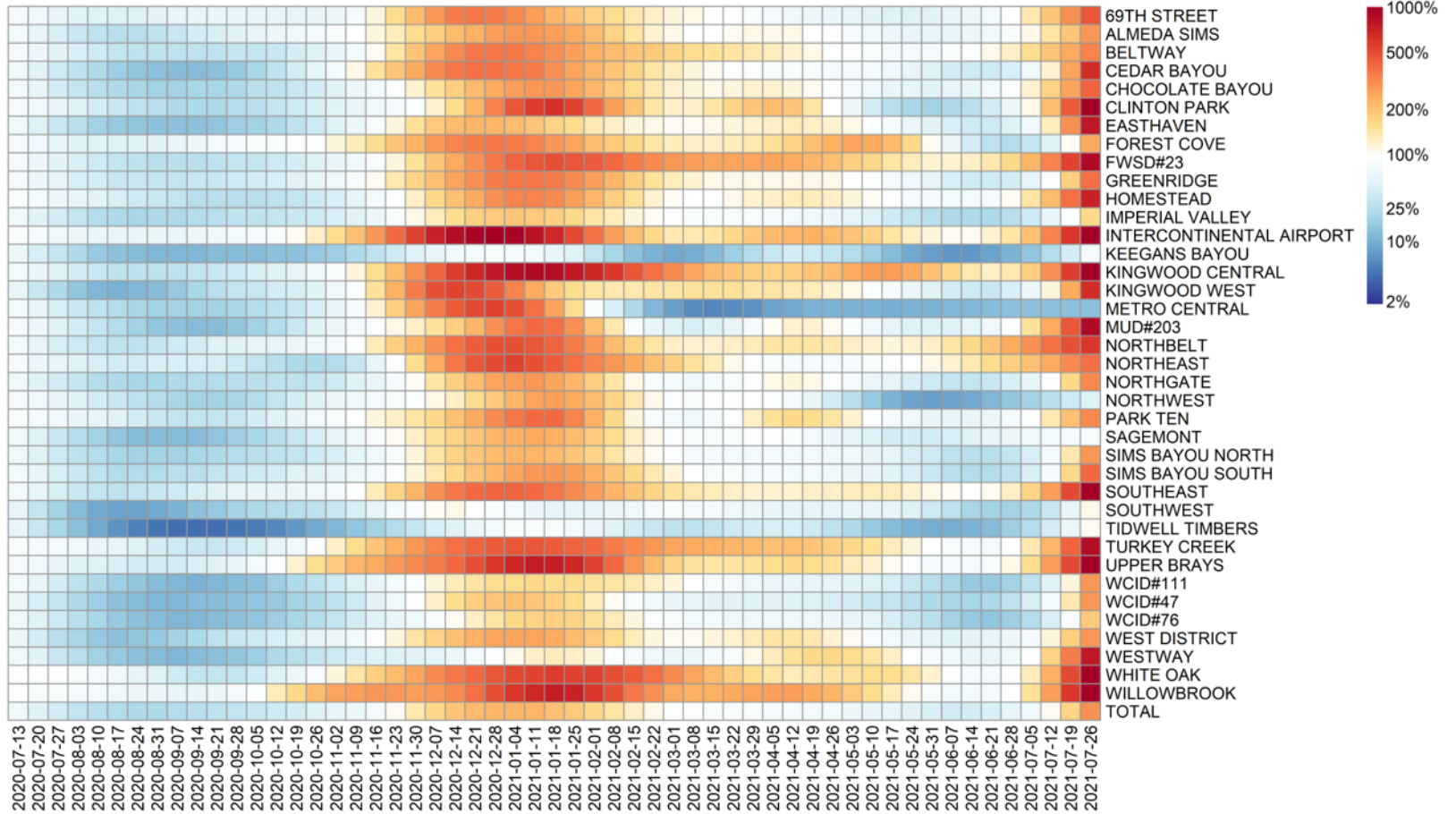
Weekly Virus Load Compared to July 6, 2020 Benchmark Levels
